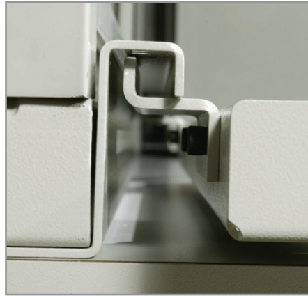
Anti-Tip Brackets
